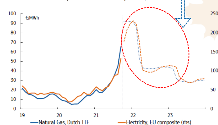
Spot and futures prices, EU
